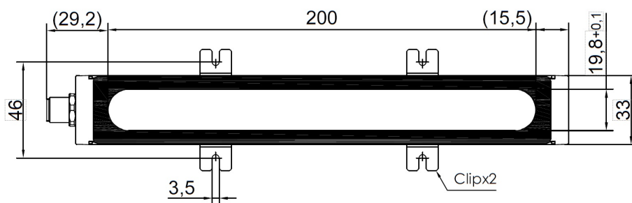
Mounting Diagram_Clip
