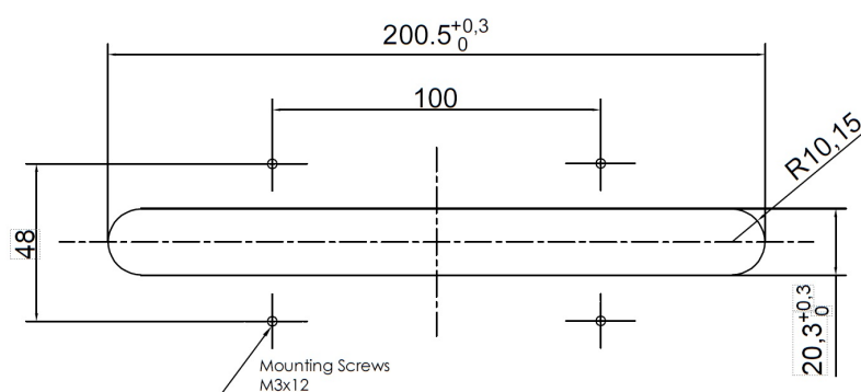
Mounting Diagram_Clip
