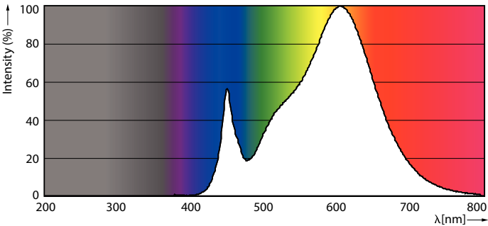
LEDcapsule CorePro 3.2-40W G9 Capsule 830 ND
