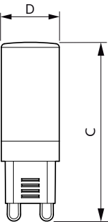
Capsule 230V3.3W-40W 370lm 3000K G9 Non
