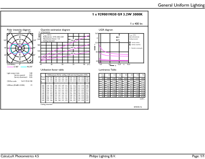
CorePro LEDcapsule ND 3.2-40W G9 830
