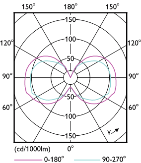
CorePro LEDcapsule ND 3.2-40W G9 830
