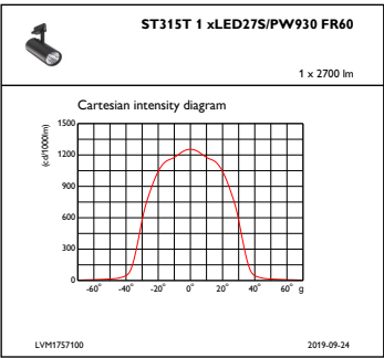
IFCC1_ST315T1xLED27SPW930FR60
