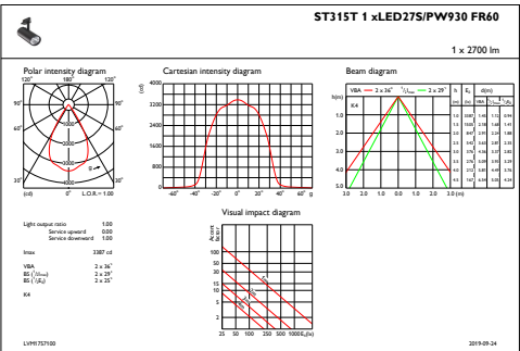
IFAS1_ST315T1xLED27SPW930FR60
