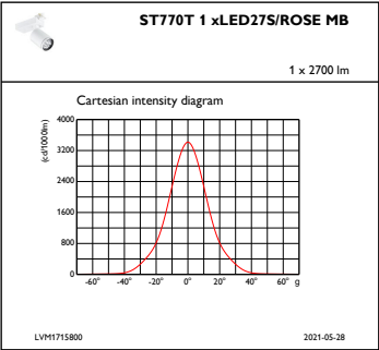
IFCC1_ST770T1xLED27SROSEMB
