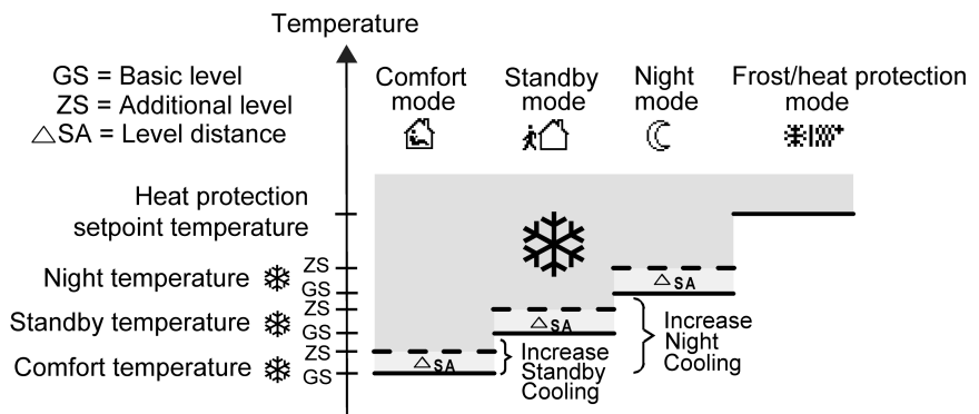
Image 46: Setpoint temperatures in the operating mode "Basic and additional cooling"
