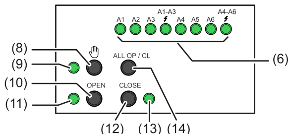
Image 4: Controls and indicators on the front panel of the device
