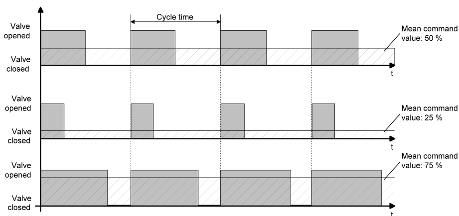
Image 10: Resulting mean value through variable duty factor with pulse width modulation
