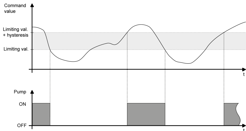
Image 8: Pump control with sample command value characteristic
