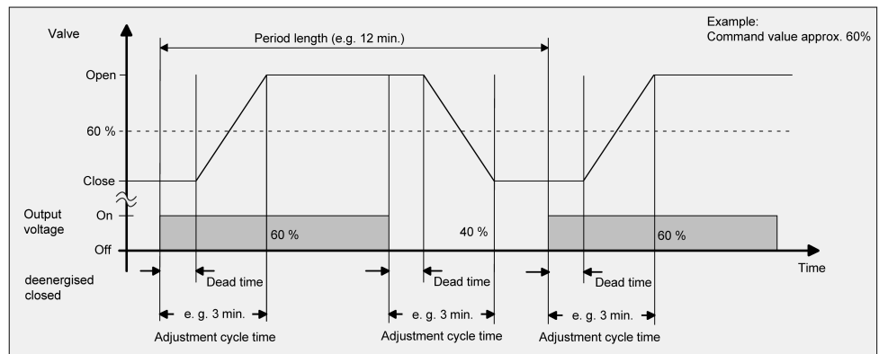
Image 18: Ideal course of the valve stroke for a cycle time > 2 x Adjusting cycle time
