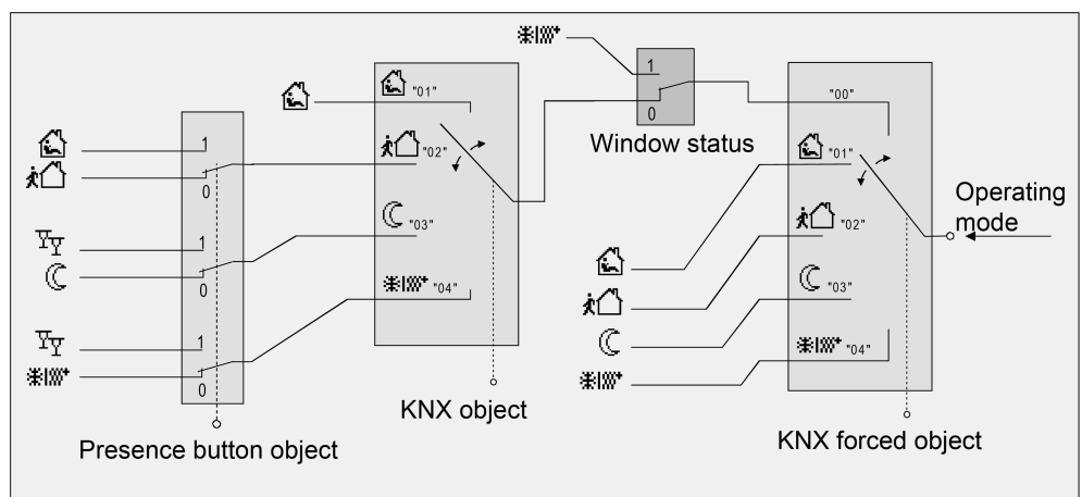
Image 41: Operating mode switchover through KNX object with presence button
