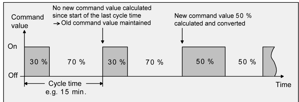
Image 32: Switching PI control
