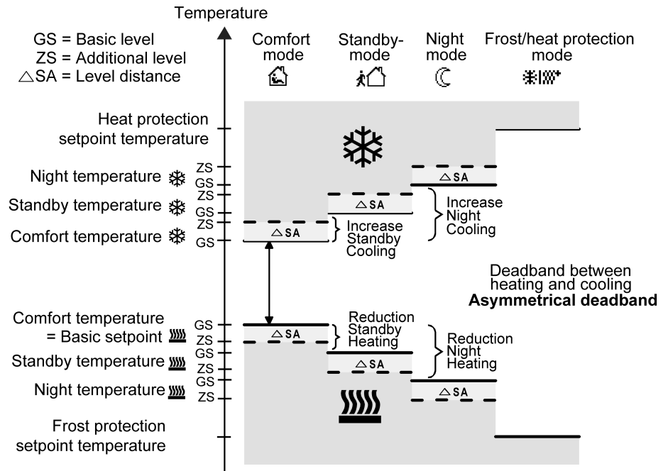
Image 50: Setpoint temperatures in the operating mode "Basic and additional heating and cooling" with asymmetrical deadband
