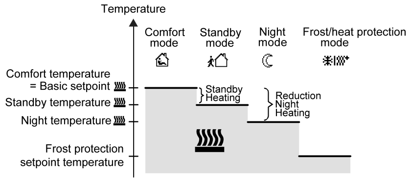
Image 43: Setpoint temperatures in the operating mode "Heating"
