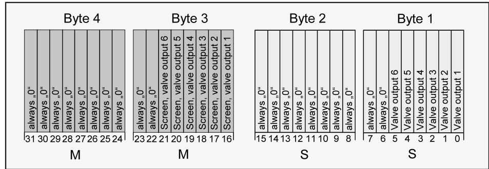
Image 5: Object structure of the collective feedback
