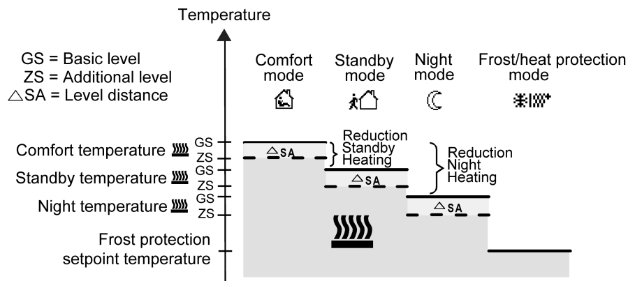
Image 44: Setpoint temperatures in the operating mode "Basic and additional heating"
