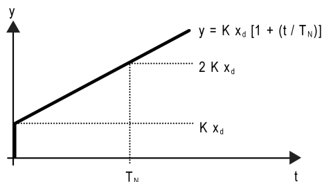
Image 37: Function of the command value of a PI control
