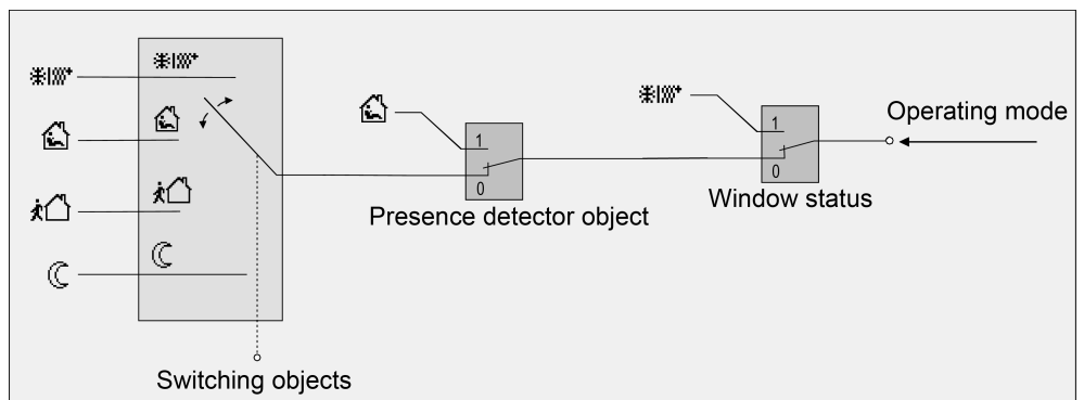
Image 40: Operating mode change-over through 4 x 1-bit objects with presence detector
