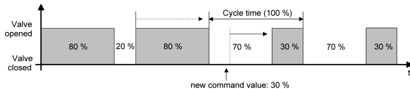
Image 12: Example of a command value change 80 % -> 30 % during the closing phase of the valve
