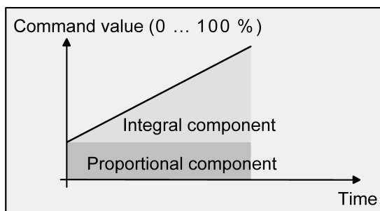
Image 31: Continuous PI control
