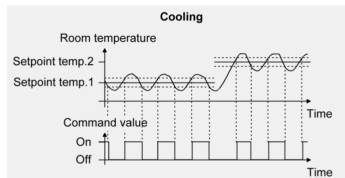
Image 34: 2-point feedback control for the single "Cooling" operating mode
