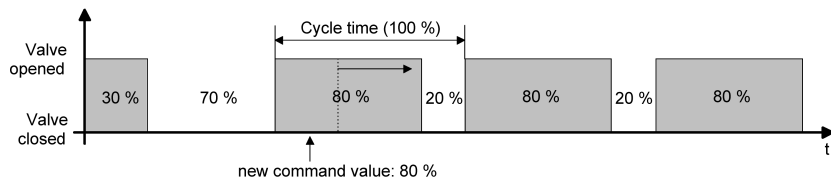
Image 14: Example of a command value change 30 % -> 80 % during the opening phase of the valve
