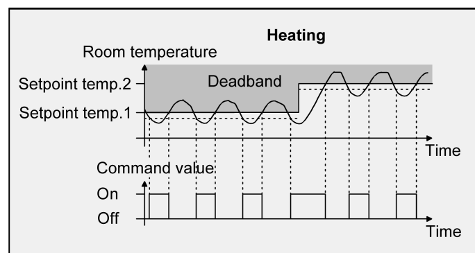
Image 35: 2-point feedback control for mixed "Heating and cooling" mode with active heating mode.
