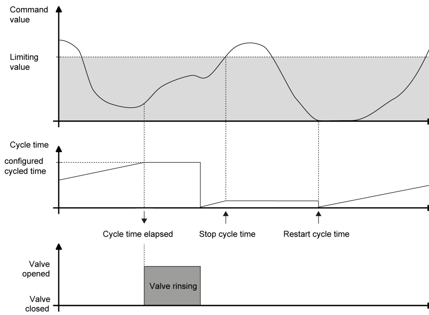
Image 28: Example of a minimum command value limiting value for intelligent valve rinsing
