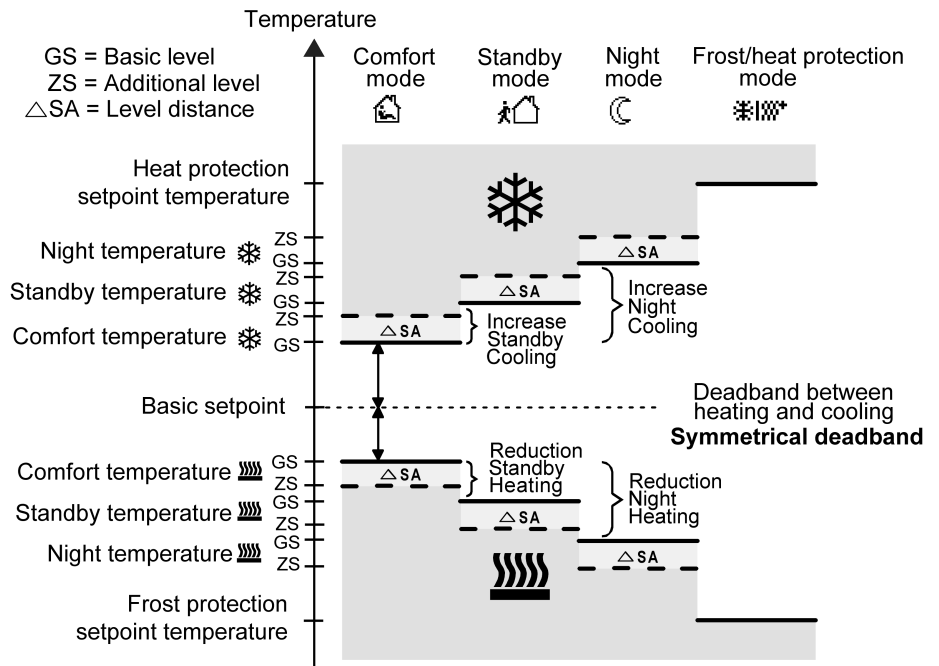
Image 49: Setpoint temperatures in the operating mode "Basic and additional heating and cooling" with symmetrical deadband
