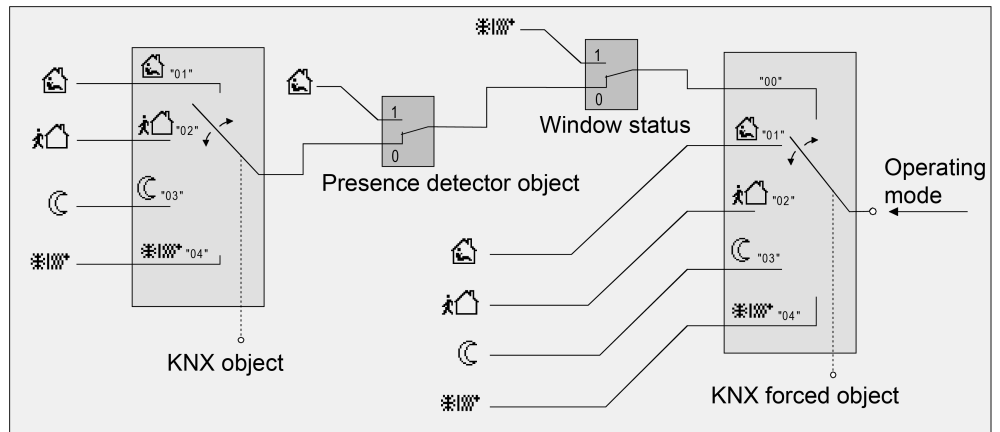
Image 42: Operating mode switchover through KNX object with presence detector
