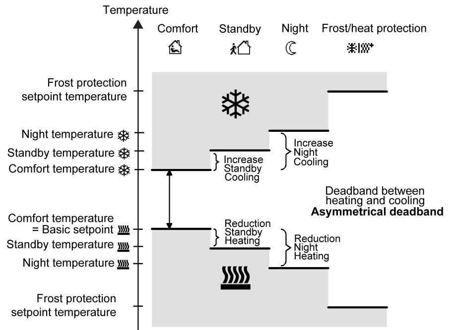
Image 48: Setpoint temperatures in the operating mode "Heating and cooling" with asymmetrical deadband
