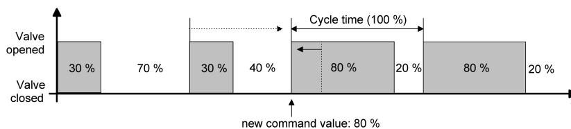
Image 16: Example of a command value change 30 % -> 80 % during the opening phase of the valve (opening phase too long)
