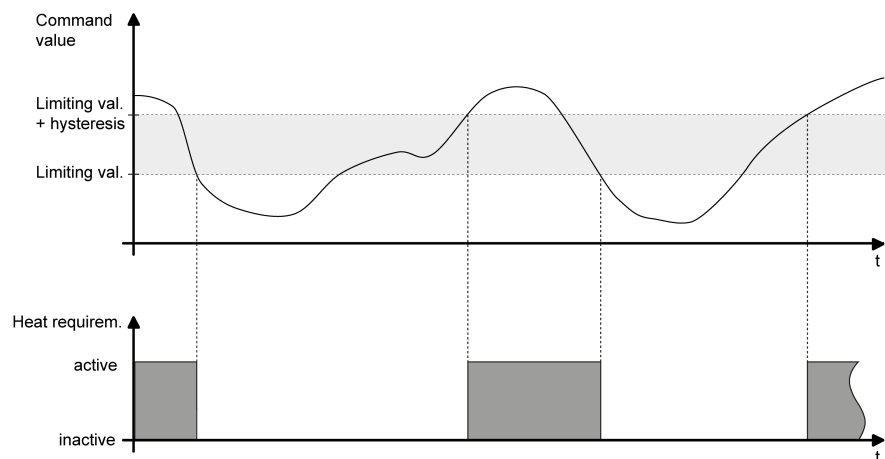
Image 7: Heat requirement information with sample command value characteristic
