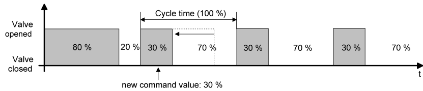
Image 11: Example of a command value change 80 % -> 30 % during the opening phase of the valve
