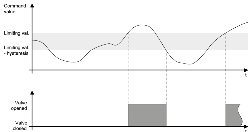
Image 17: Example of command value evaluation with limiting value
