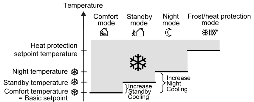
Image 45: Setpoint temperatures in the operating mode "Cooling"
