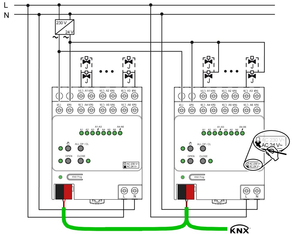
Image 3: Connection for actuators AC 24 V
