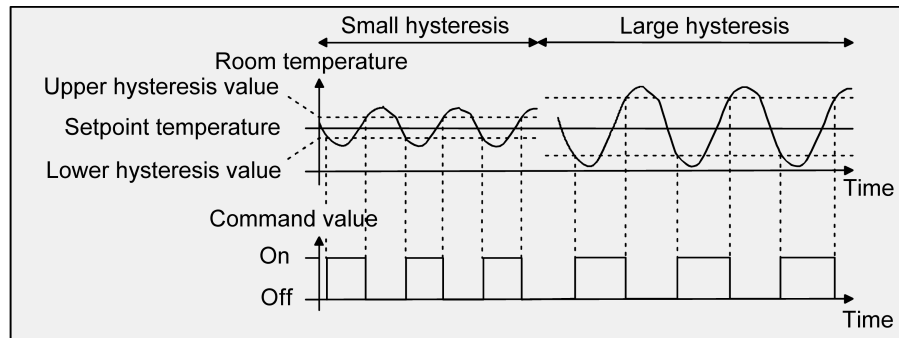
Image 38: Effects of the hysteresis on the switching behaviour of a 2-point feedback control command value
