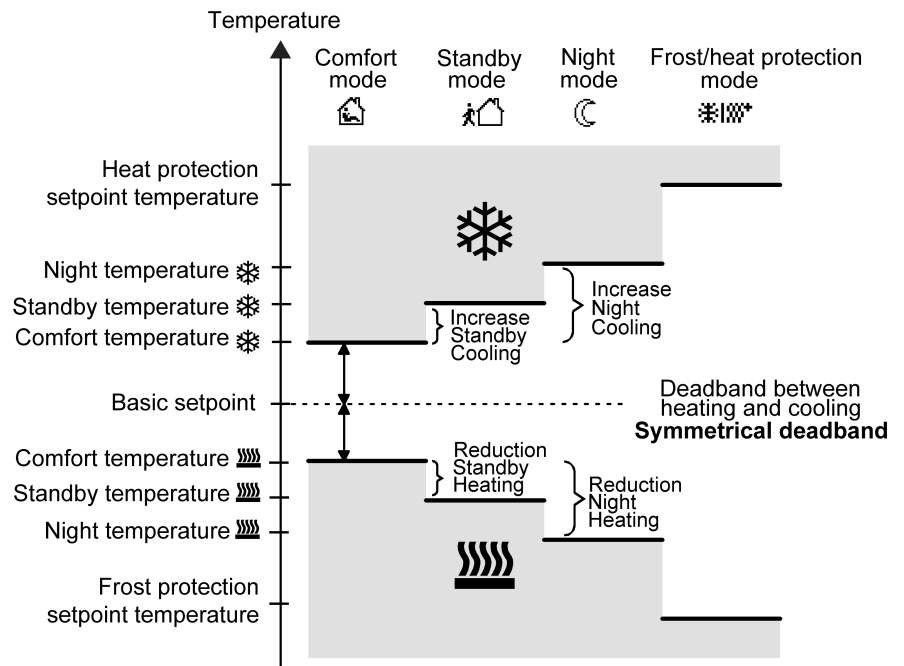
Image 47: Setpoint temperatures in the operating mode "Heating and cooling" with symmetrical deadband
