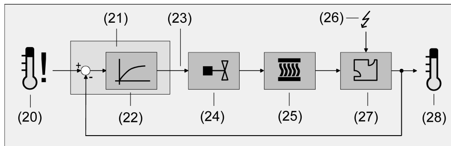
Image 30: Controlled system of single-room temperature control
