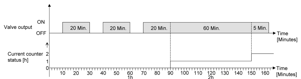
Image 29: Function of the operating hours counter (using the example of an up-counter)
