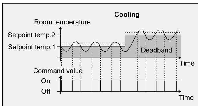
Image 36: 2-point feedback control for mixed "Heating and cooling" mode with active cooling operation.
