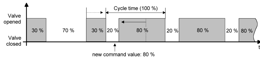
Image 15: Example of a command value change 30 % -> 80 % during the closing phase of the valve
