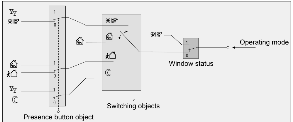
Image 39: Operating mode change-over through 4 x 1-bit objects with presence button
