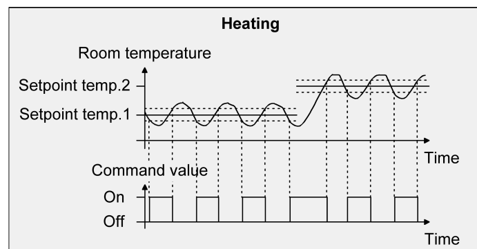
Image 33: 2-point feedback control for the single "Heating" operating mode
