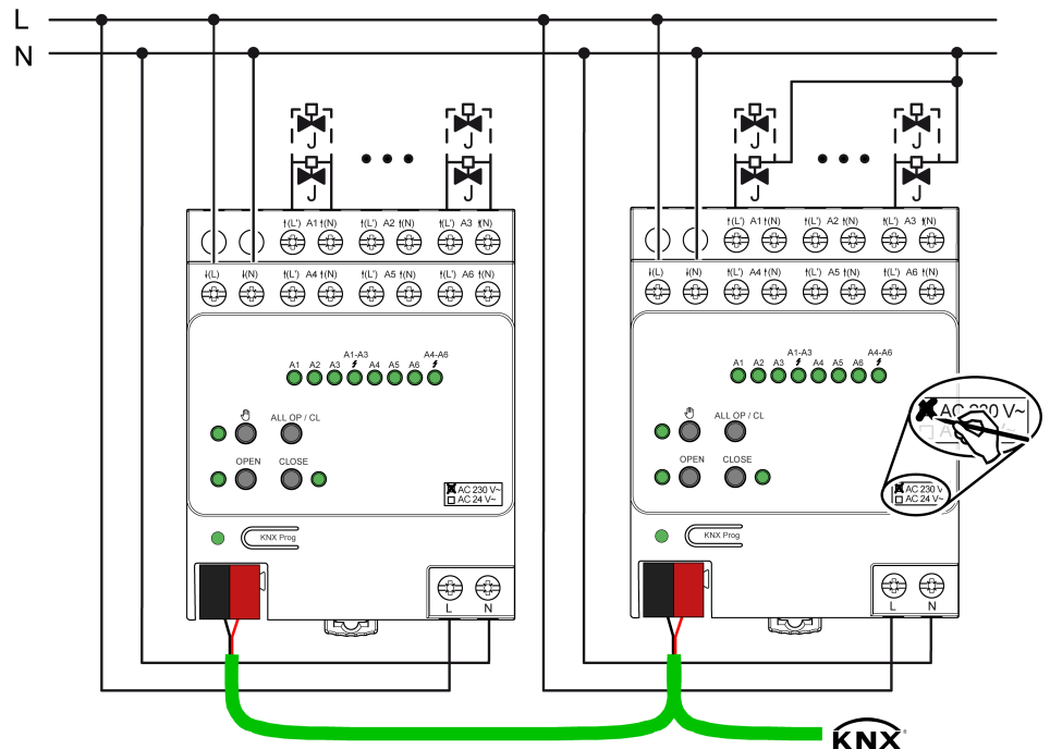
Image 2: Connection for AC 230 V actuators (connection examples) Left: Neutral conductor of the actuators run separately to the actuator / Right: Shared neutral conductor for actuators
