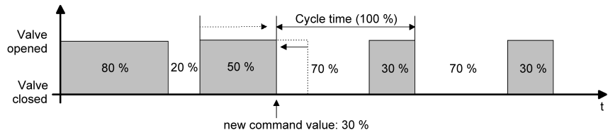
Image 13: Example of a command value change 80 % -> 30 % during the opening phase of the valve (opening phase too long)
