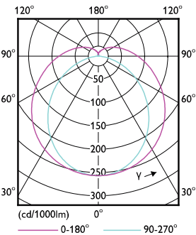
TLED_4ft_220-240V15.5-36W_G13-LDD
