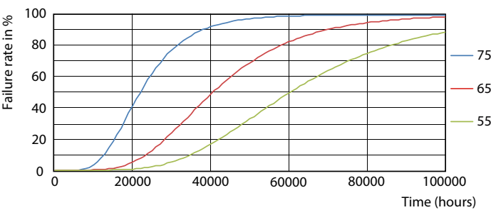
TLED_220-240V_G13-FailureRate
