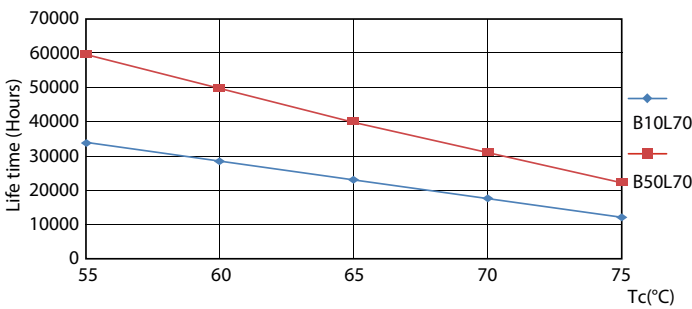
TLED_220-240V_G13-LifetimeVsTc
