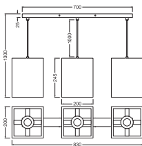
DECOR CARDBOARD SQUARE PEND 3XE27
