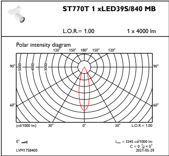
OFPC1_ST770T1xLED39S840MB
