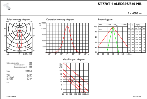
IFAS1_ST770T1xLED39S840MB
