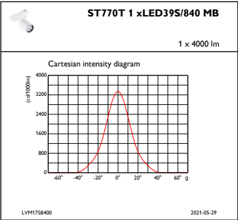
IFCC1_ST770T1xLED39S840MB
