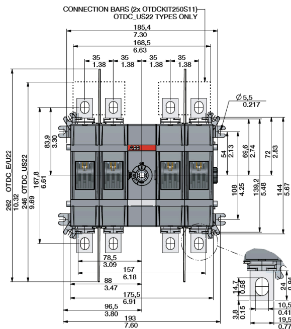
OTDC100...250E22, OTDC100...200U22
