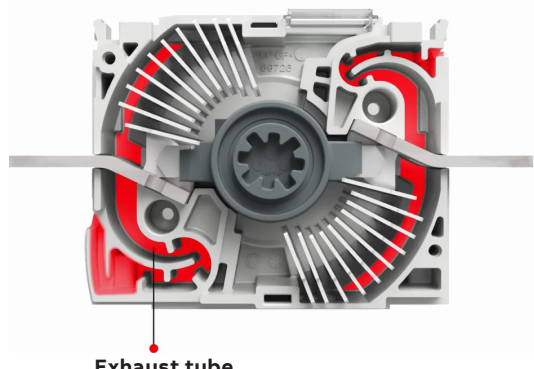
Exhaust tube
