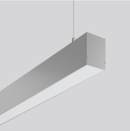
Pendelarmaturen 4068754003599 L 1687, B 57, H 75 pendelmontage zilver, mat (ca. RAL 9006)
