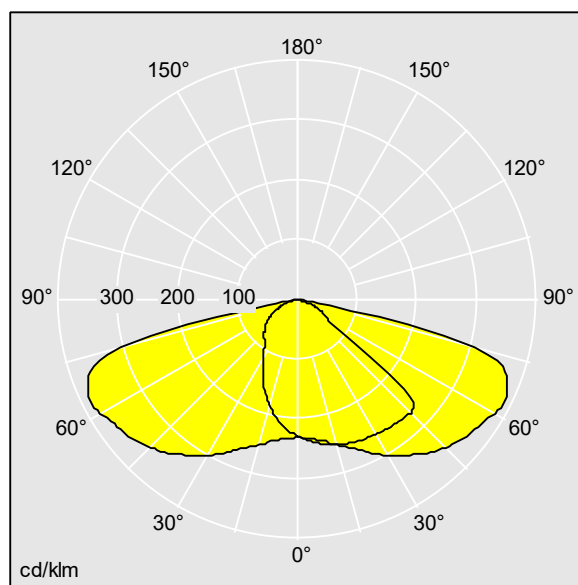
TL_CTS24L105NR730.ltd
