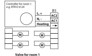
Valve for room 1
