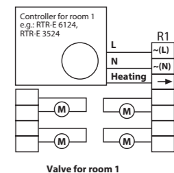
Valve for room 1
