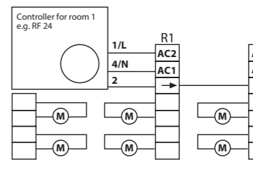
Valve for room 1 Additional valve for room 1
