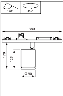
ST770X 27S/840 DIA VWB FG WH
