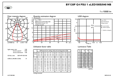
IFGU1_BY120PG4PSU1xLED100S840NB
