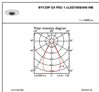
IFPC1_BY120PG4PSU1xLED100S840NB
